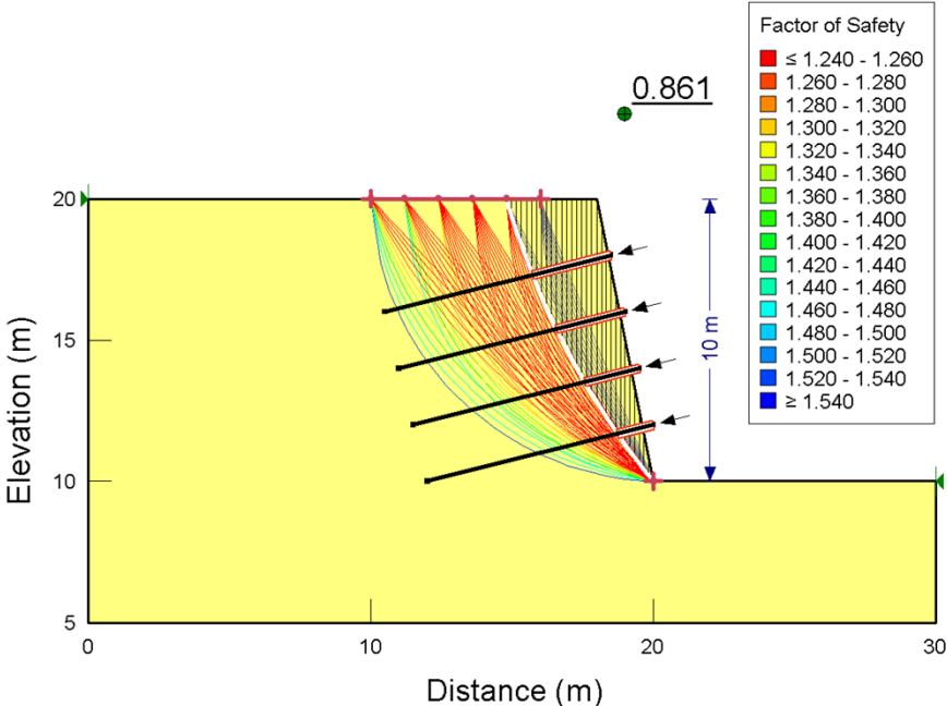
Figure 7. Critical Slip Surface for Case 3.
