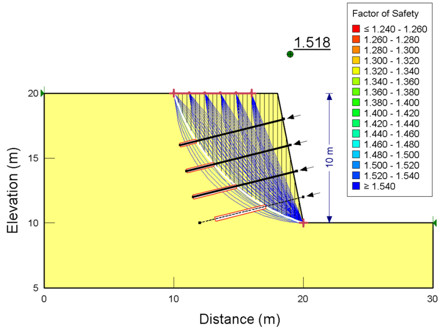
Figure 6. Critical Slip Surface for Case 2.
