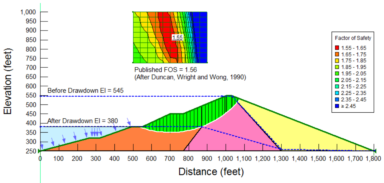
Figure 4 SLOPE/W Computed Factor of Safety Using the 3 Stage Undrained Strength Method
