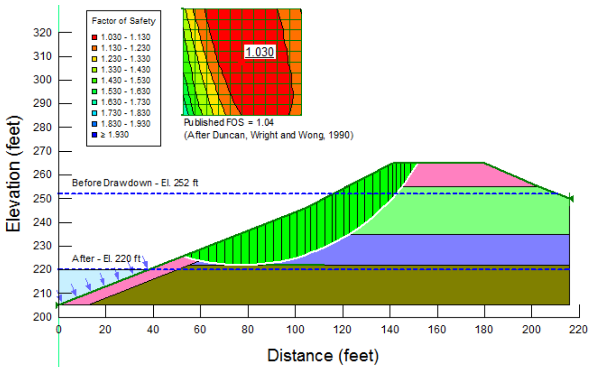
Figure 2 SLOPE/W Computed Factor of Safety Using the 3-Stage Undrained Strength Method
