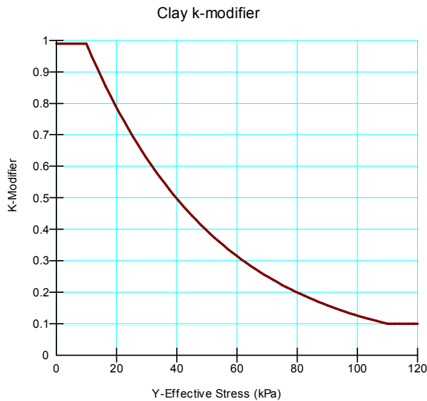
Figure 5 An illustrative conductivity (K) modifier function
