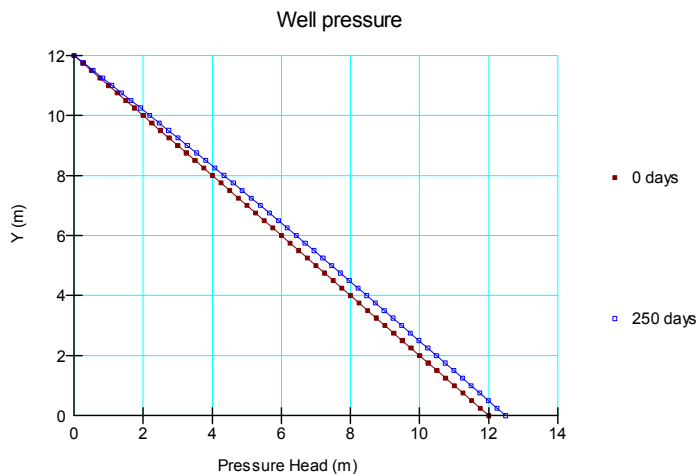
Figure 12 Excess pressure head distribution in the well
