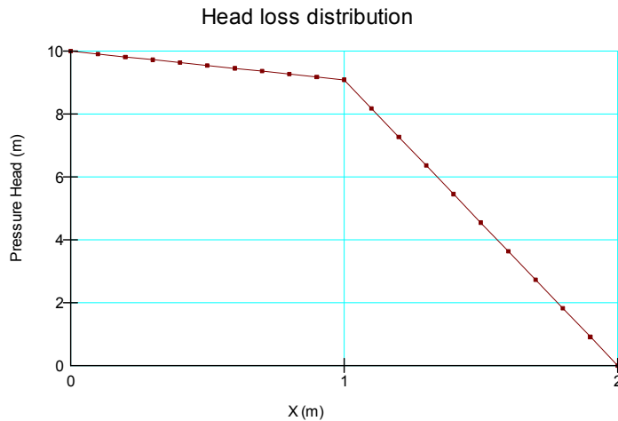
Figure 4 Head loss distribution in a layered system
