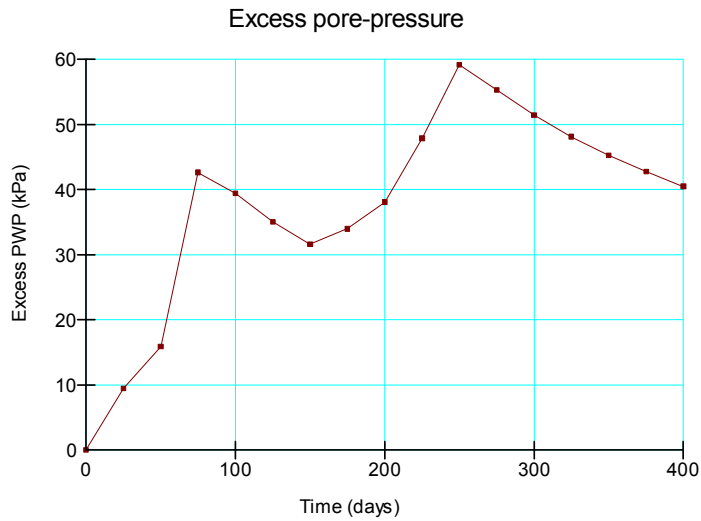
Figure 10 Excess pore-pressures at the mid-way point between two drains at the contact between the very soft clay and the underlying slightly more competent clay (EI 5 m)
