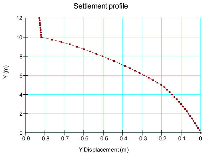
Figure 9 Settlement profile at the end of 400 days
