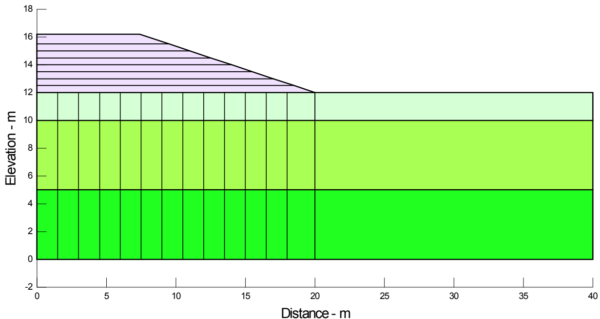
Figure 2 Position of the vertical drains and layers used for sequential fill placement
