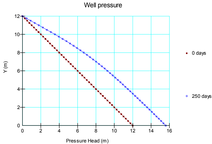
Figure 13 Excess pressure head distribution in the well with a reduced conductivity
