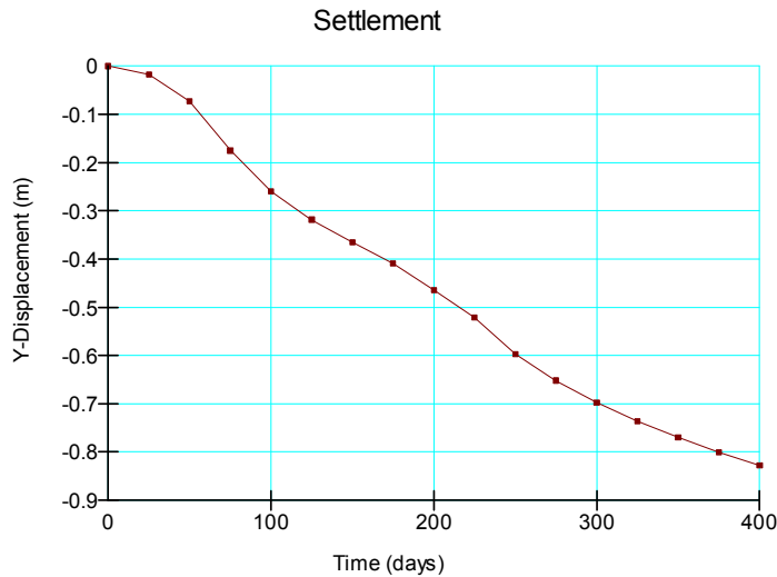
Figure 8 Surface settlement with 1.5 m drain spacing
