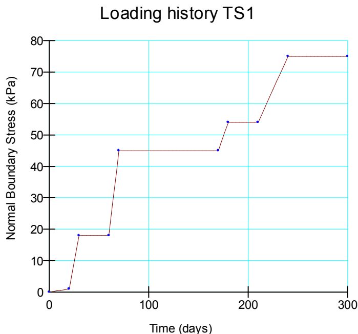
Figure 7 Applied pressure to represent the embankment fill placement
