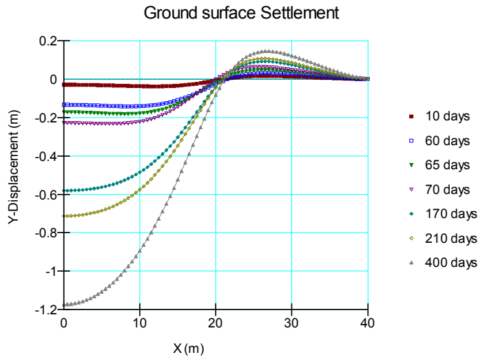
Figure 14 Ground surface settlement profiles
